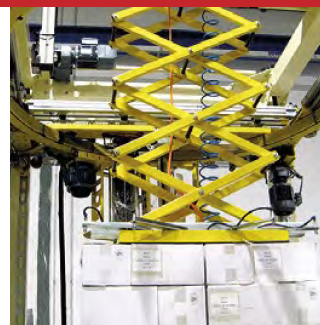
Motorized hold down plate
