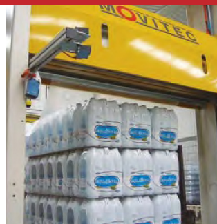
Independent top sheet dispenser
