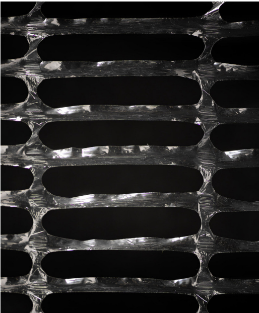
AFTER elongation (MIN 100mm)
